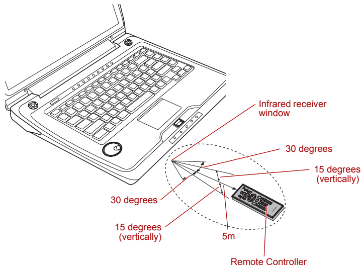
Figure 8-5 Operational range of the remote control
